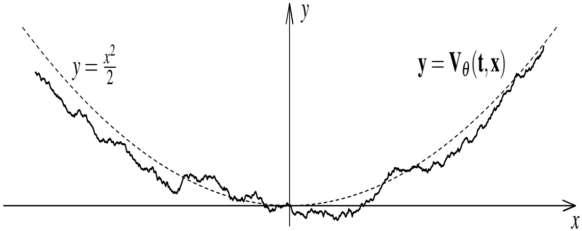
Figure 3.1: Realization of the random potential freezed at time t
